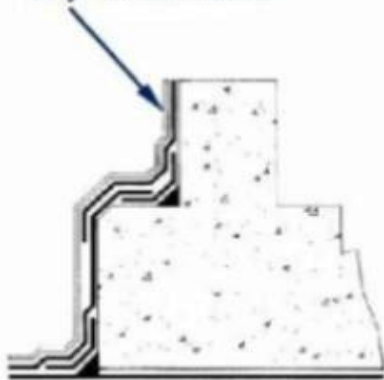
10mm Bitubond Cork Heavy Duty Protection Board
