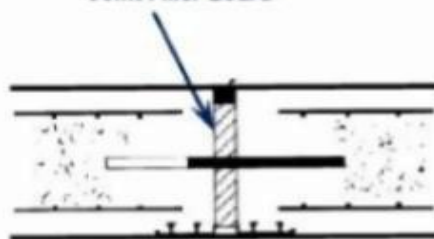
Bitubond Cork Heavy Duty Joint Filler Board
